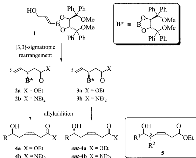
Scheme 1. Synthesis of new enantiomerically pure reagents 2 and 3 for allylations by a [3,3] sigmatropic rearrangement
