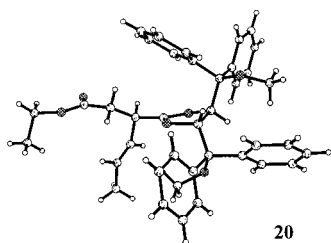
Scheme 5. Synthesis of crotylboronic esters 19 and 20 ; the absolute configuration of reagent 20 was established by X-ray structural analysis
