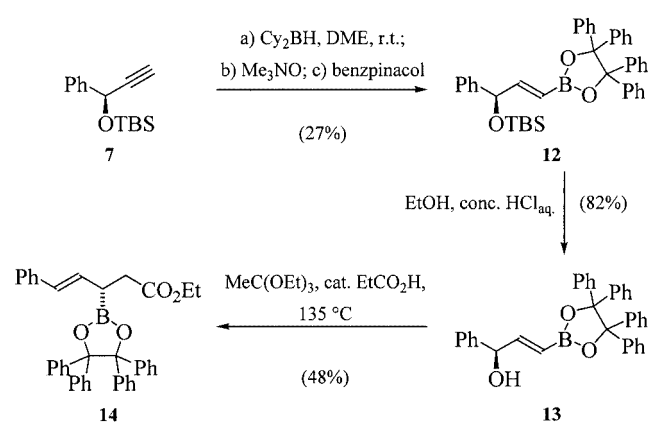
Scheme 3. Synthesis of benzpinacol-derived allylboronic ester 14
