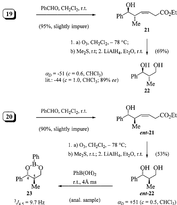
Scheme 6. Allyl additions of reagents 19 and 20 ; the absolute and relative configurations of homoallyl alcohol 21/ent - 21 was established by chemical correlation with known diol 22/ent - 22 and dioxaborinane 23
