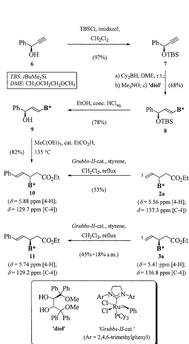
Scheme 2. Synthesis of allylboronic esters 10 and 11 ; determination of their absolute configurations
