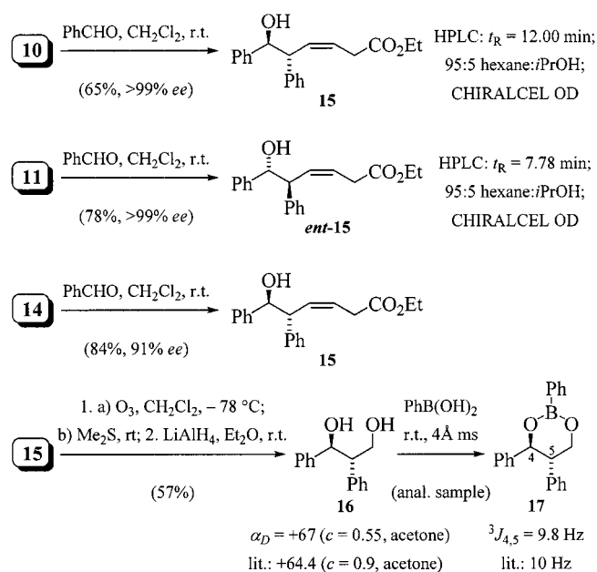
Scheme 4. Allyl additions of reagents 10 , 11 and 14 ; the absolute and relative configuration of homoallyl alcohol 15 was established by chemical correlation with known diol 16 and dioxaborinane 17
